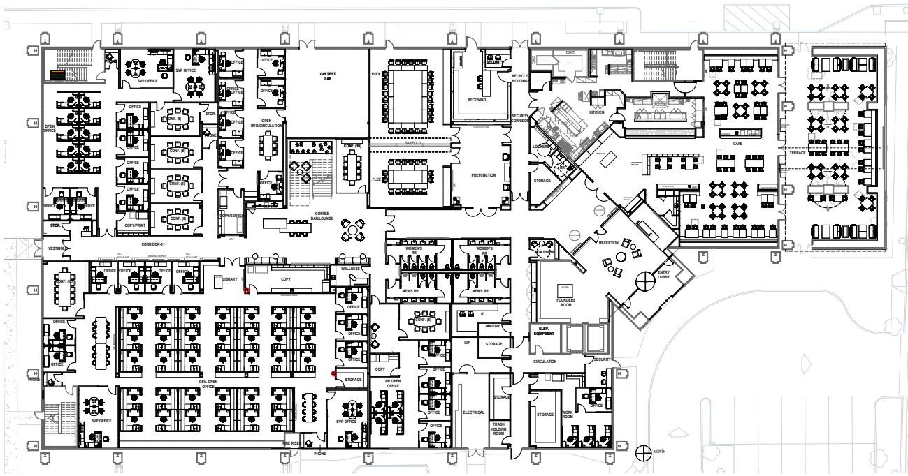
LEVEL 01 FLOOR PLAN LAYOUT
